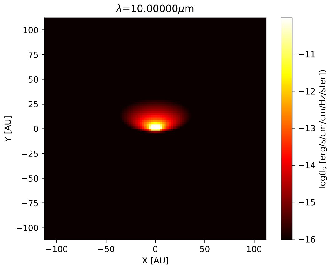
Fig. 8.12: The rectangular ('normal') version of the image of Fig. 8.11. As one can see: the inner regions of this image are not well-resolved.
